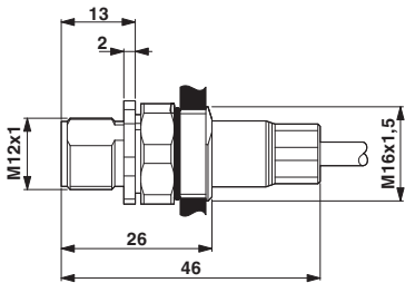
M12 flush-type plug, front mounting, can be positioned
